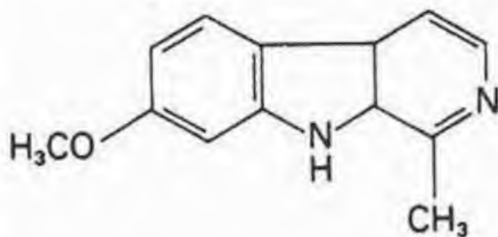
HARMINE
